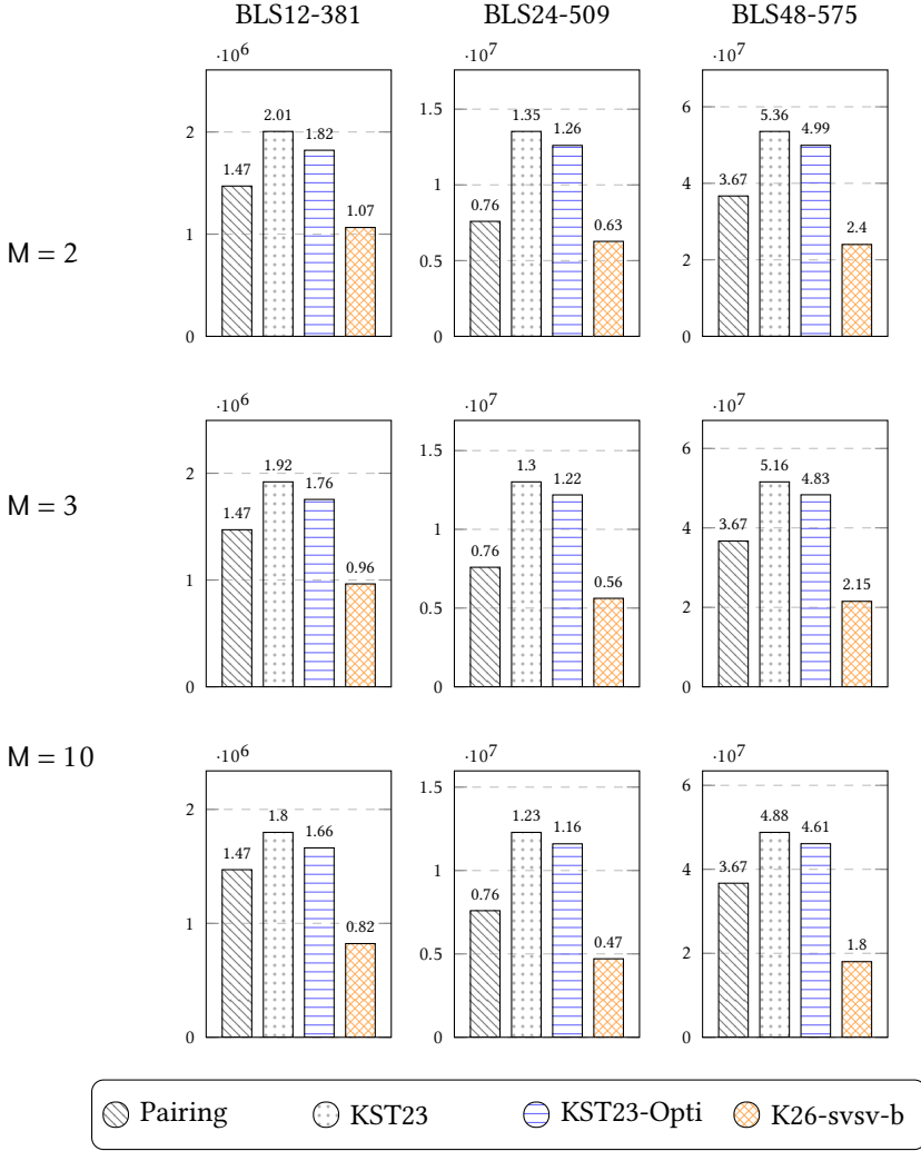
Figure 5.4: Batch pairing delegation cost comparison for type SVSV.
