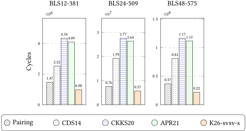
Figure 5.3: Single pairing delegation cost comparison for type SVSV.
